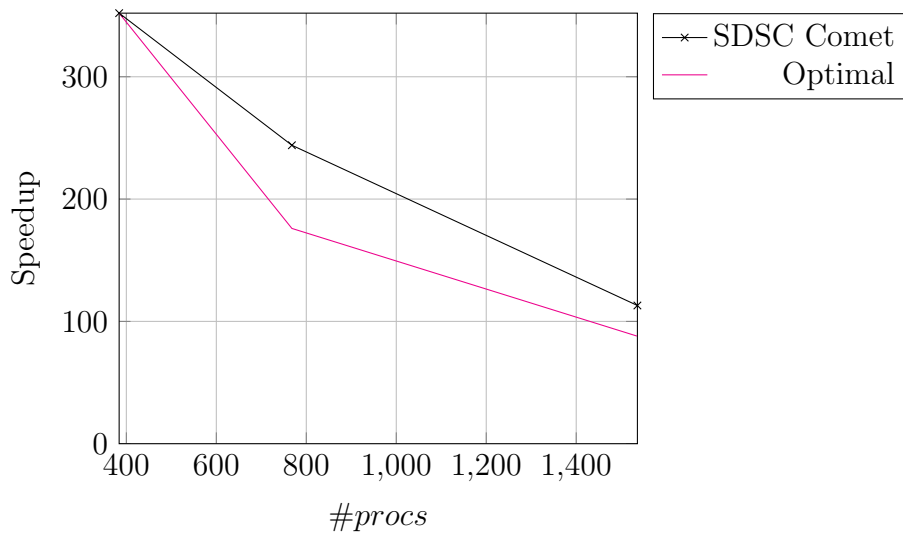
Figure 6: Strong scaling result for the subproject whole-cell calcium dynamics. Scaled speedup of distributed execution, where \#procs denotes the involved processes on SDSC Comet, demonstrate scaling behavior. Problem sizes are illustrated in Table ??.
